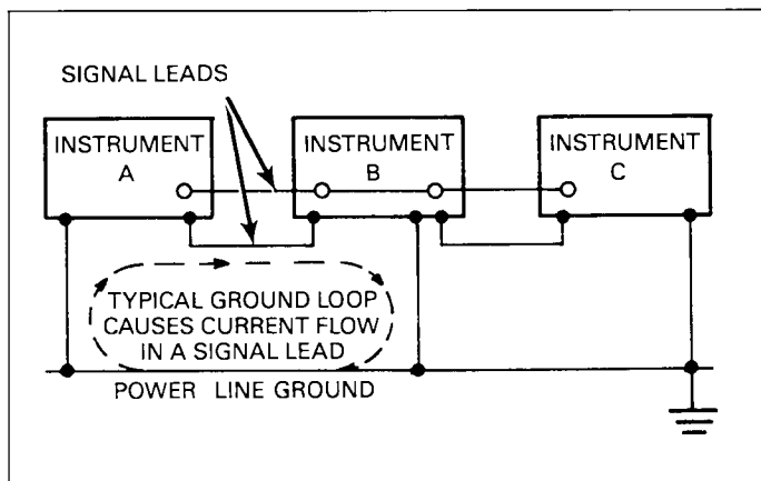
Figure 2-32. Multiple Ground Points Create a Ground Loop
